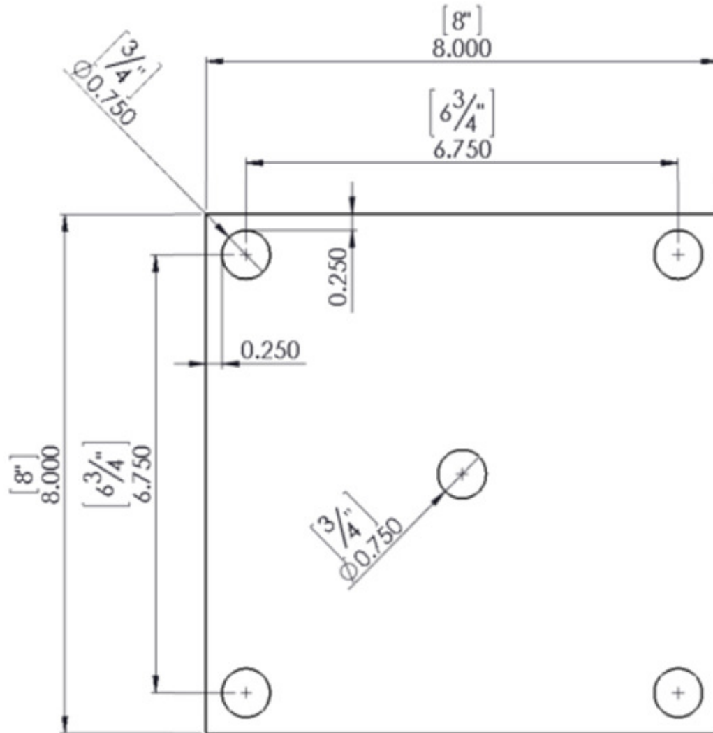
3/8" Plate
